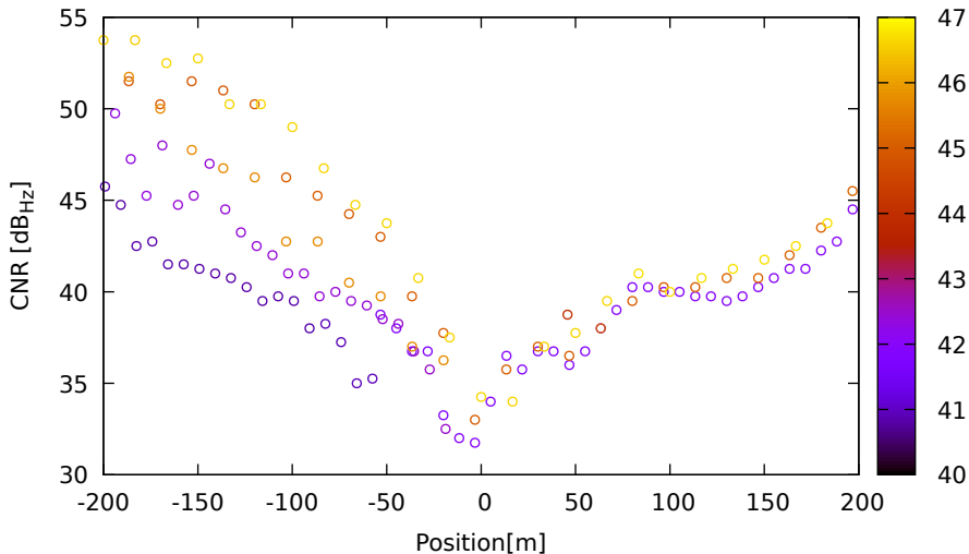
CNR vs position for E05 (E8) on LeicaGS18 - DOY 262 jam. 1
