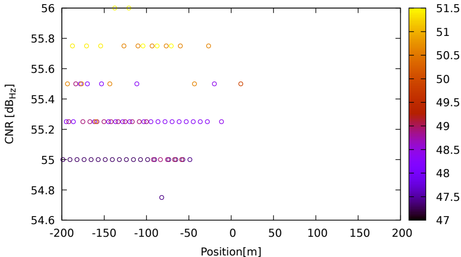
CNR vs position for E05 (E8) on LeicaGS18 - DOY 262 jam. 2
