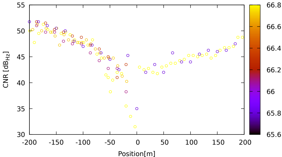
CNR vs position for E09 (E1) on LeicaGS18 - DOY 262 jam. 1
