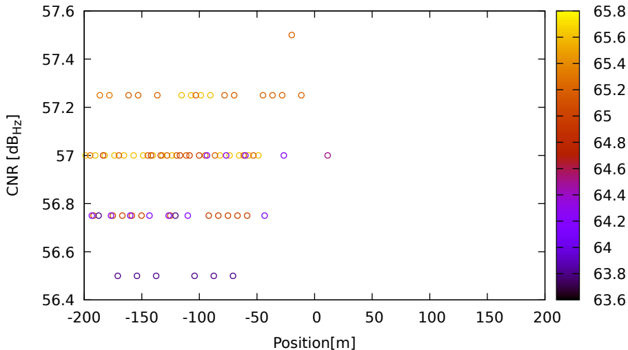
CNR vs position for E09 (E8) on LeicaGS18 - DOY 262 jam. 2
