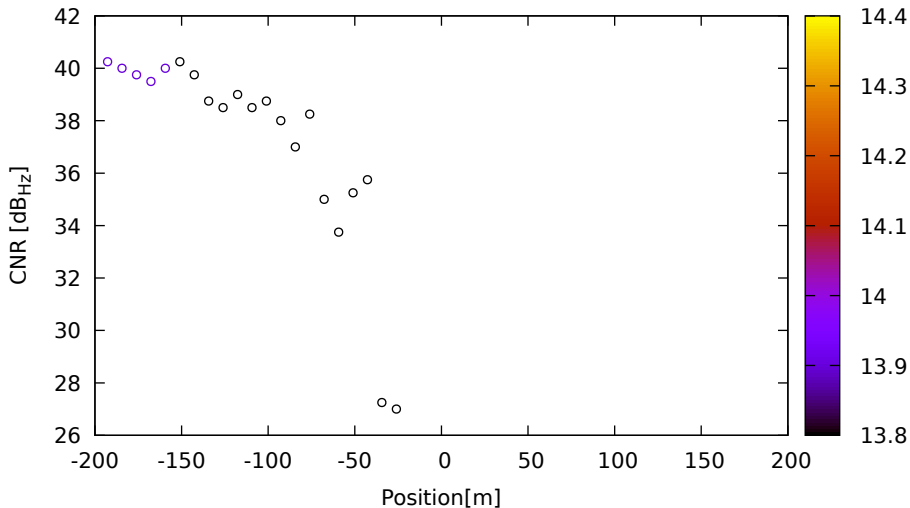
CNR vs position for E11 (E1) on LeicaGS18 - DOY 262 jam. 3
