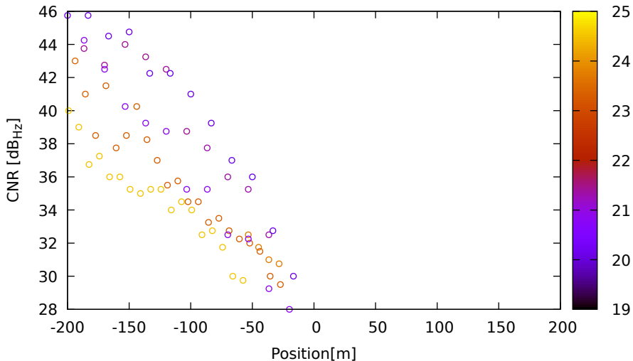
CNR vs position for E11 (E8) on LeicaGS18 - DOY 262 jam. 1
