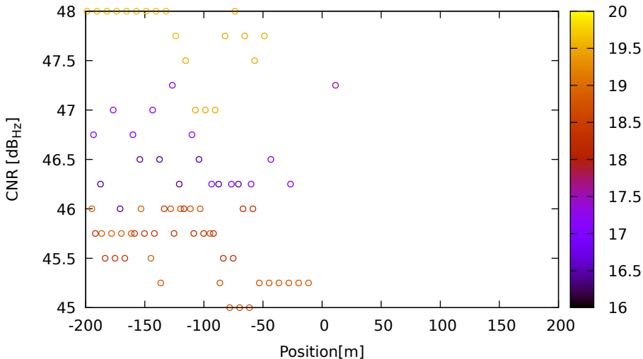
CNR vs position for E11 (E8) on LeicaGS18 - DOY 262 jam. 2
