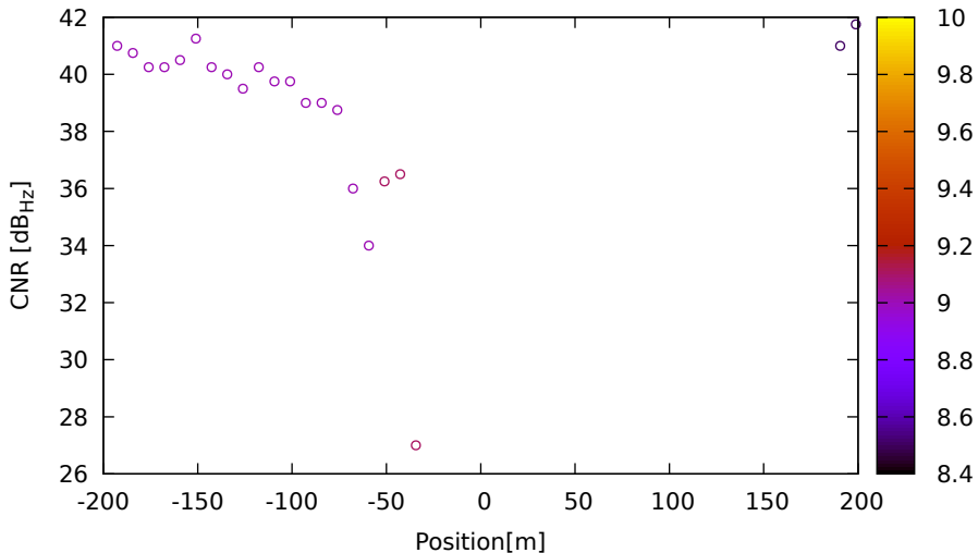
CNR vs position for E15 (E1) on LeicaGS18 - DOY 262 jam. 3
