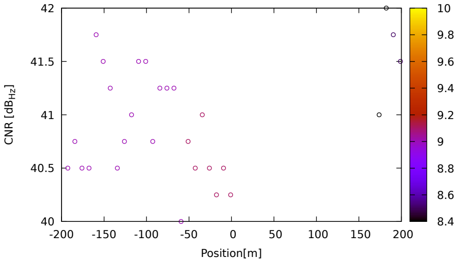
CNR vs position for E15 (E5b) on LeicaGS18 - DOY 262 jam. 3
