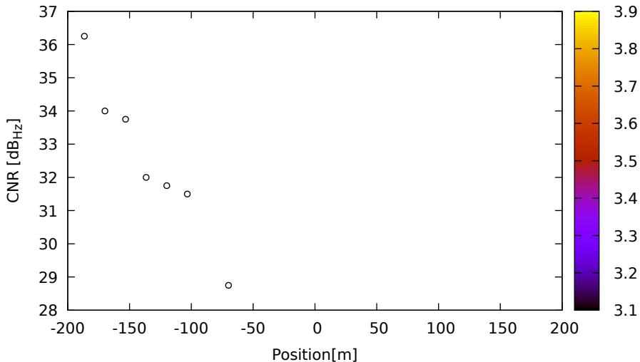
CNR vs position for E27 (E1) on LeicaGS18 - DOY 262 jam. 1
