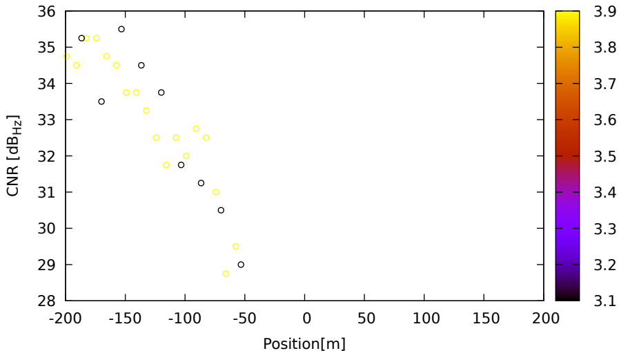
CNR vs position for E27 (E5a) on LeicaGS18 - DOY 262 jam. 1
