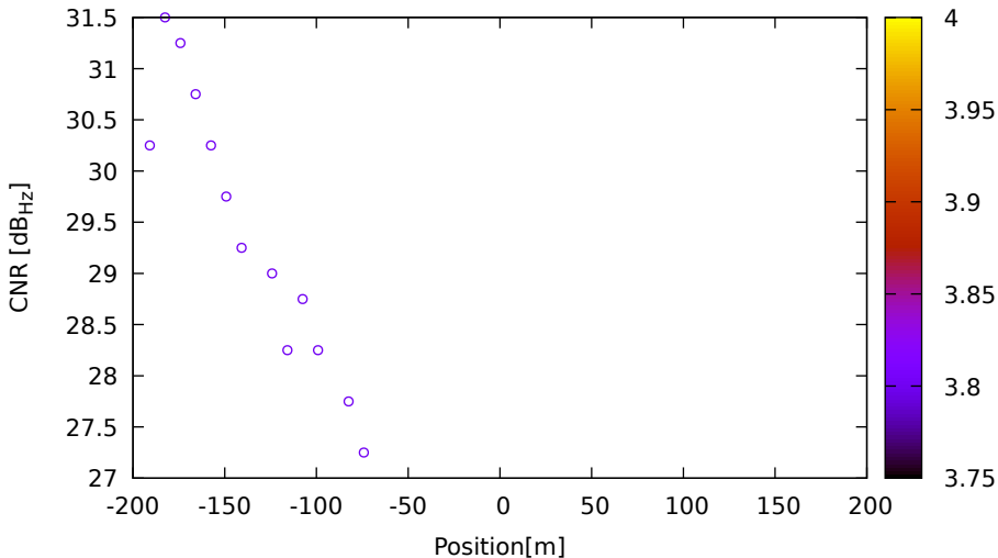
CNR vs position for E30 (E5a) on LeicaGS18 - DOY 262 jam. 1
