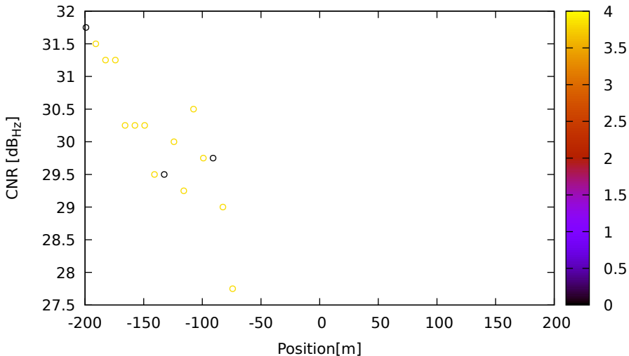
CNR vs position for E30 (E5b) on LeicaGS18 - DOY 262 jam. 1
