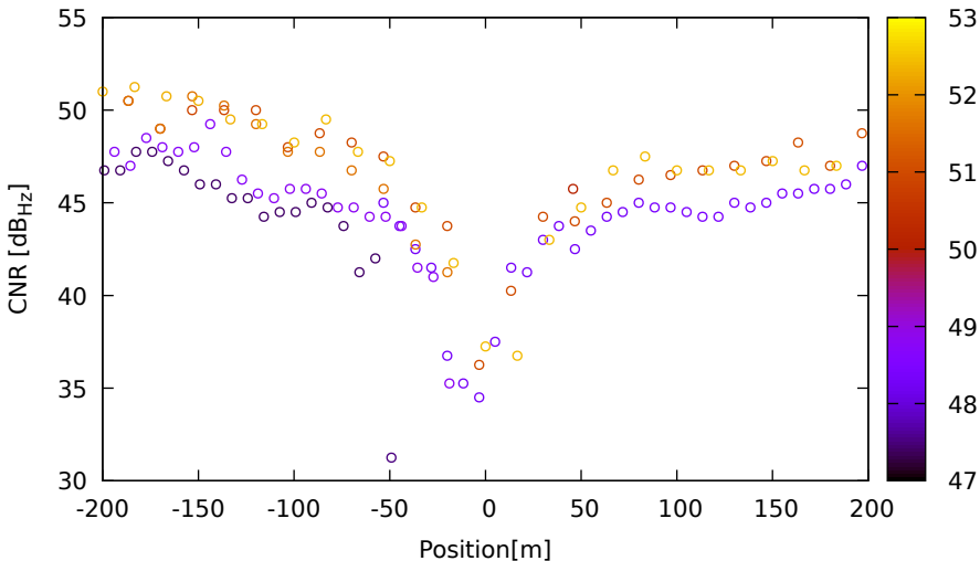
CNR vs position for E34 (E5a) on LeicaGS18 - DOY 262 jam. 1
