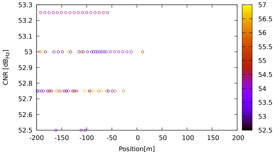
CNR vs position for E34 (E5a) on LeicaGS18 - DOY 262 jam. 2
