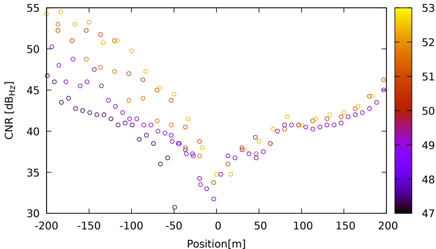
CNR vs position for E34 (E8) on LeicaGS18 - DOY 262 jam. 1
