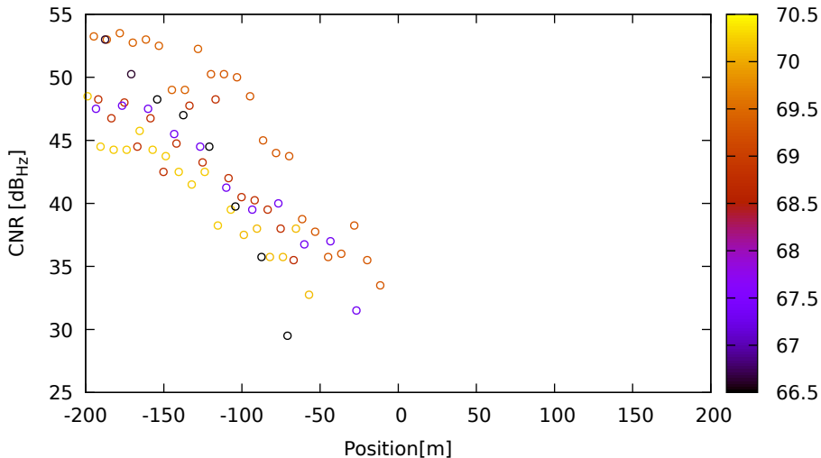
CNR vs position for E36 (E1) on LeicaGS18 - DOY 262 jam. 2
