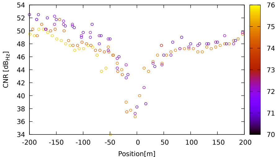
CNR vs position for E36 (E5a) on LeicaGS18 - DOY 262 jam. 1
