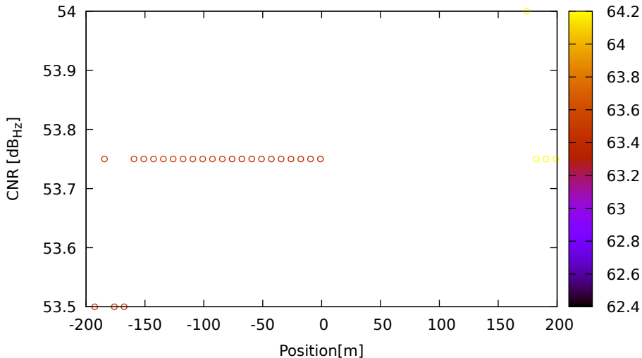
CNR vs position for E36 (E5a) on LeicaGS18 - DOY 262 jam. 3
