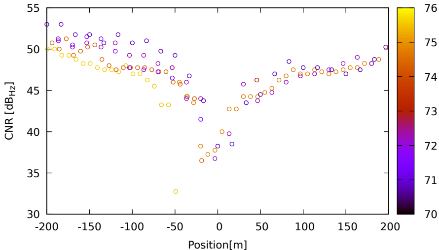
CNR vs position for E36 (E5b) on LeicaGS18 - DOY 262 jam. 1
