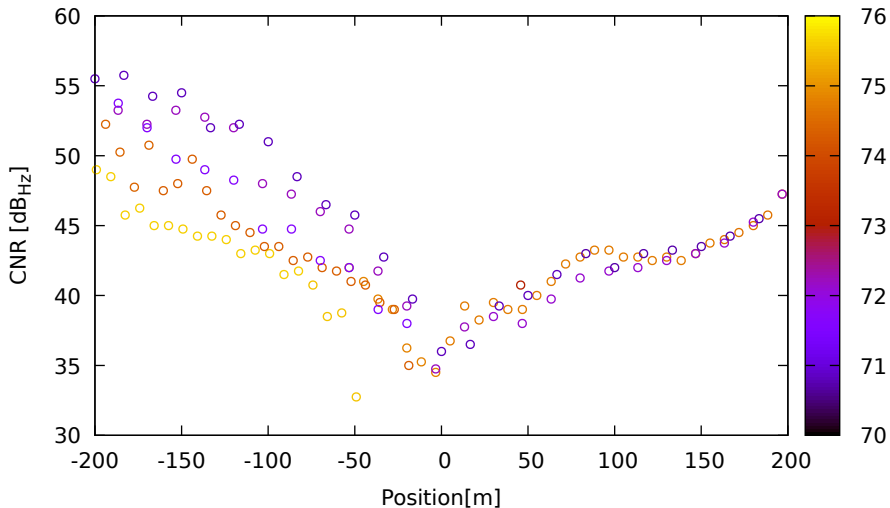
CNR vs position for E36 (E8) on LeicaGS18 - DOY 262 jam. 1
