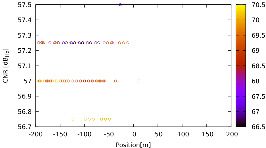
CNR vs position for E36 (E8) on LeicaGS18 - DOY 262 jam. 2
