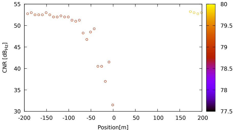
CNR vs position for G01 (L1) on LeicaGS18 - DOY 262 jam. 3
