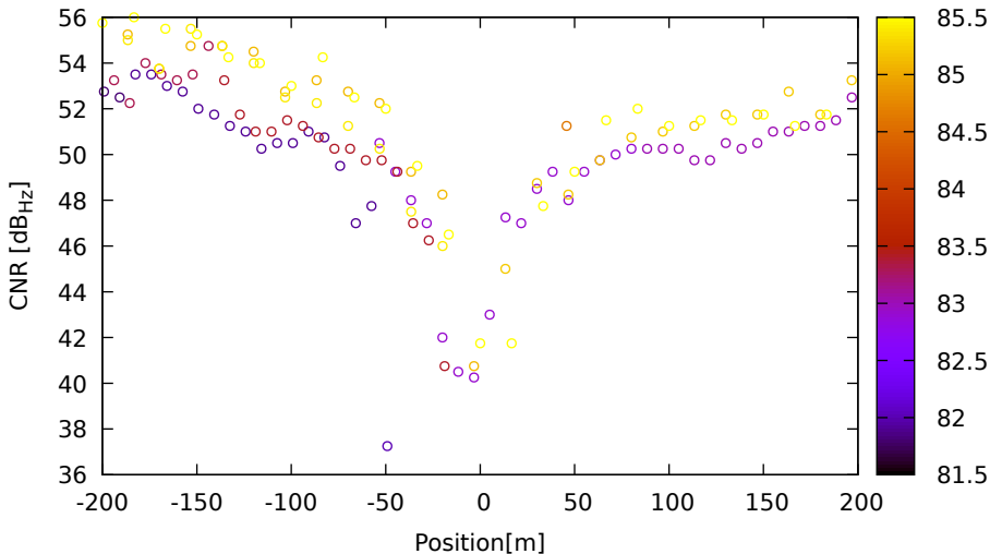
CNR vs position for G01 (L5) on LeicaGS18 - DOY 262 jam. 1
