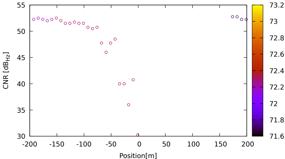
CNR vs position for G03 (L1) on LeicaGS18 - DOY 262 jam. 3
