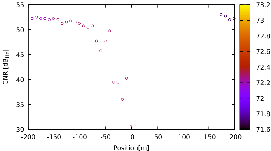
CNR vs position for G03 (L2) on LeicaGS18 - DOY 262 jam. 3
