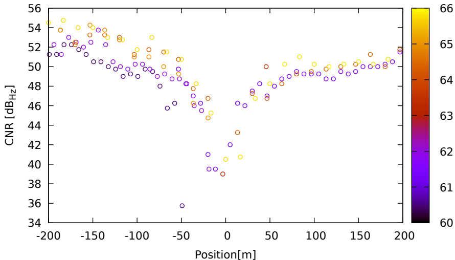
CNR vs position for G03 (L5) on LeicaGS18 - DOY 262 jam. 1
