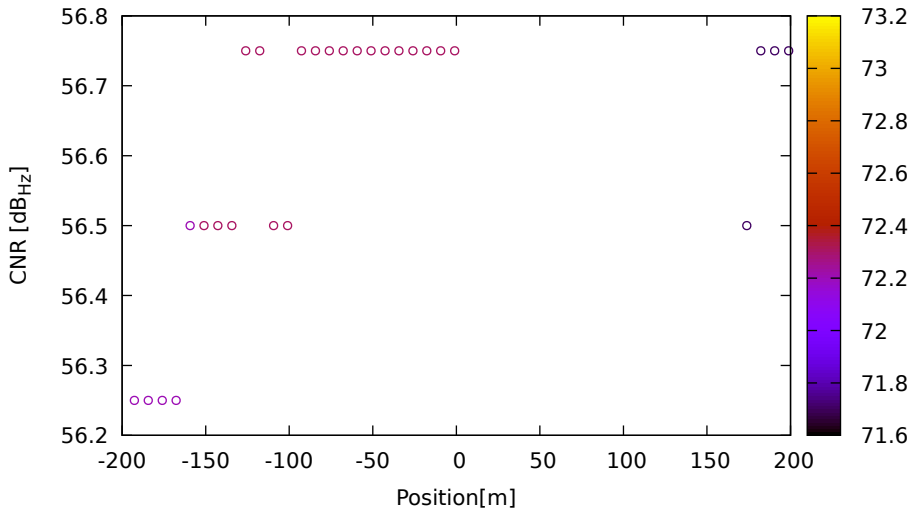
CNR vs position for G03 (L5) on LeicaGS18 - DOY 262 jam. 3
