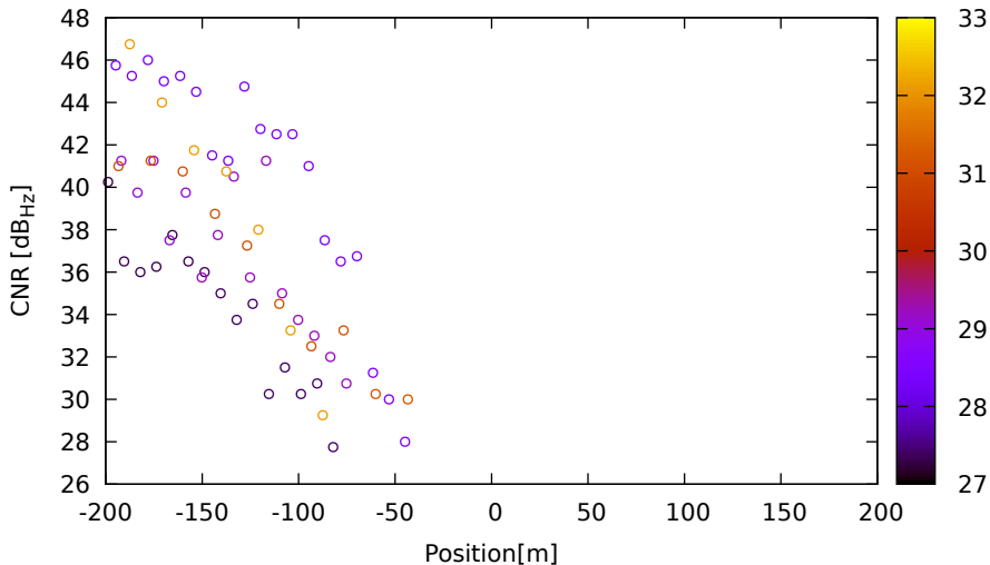
CNR vs position for G04 (L1) on LeicaGS18 - DOY 262 jam. 2
