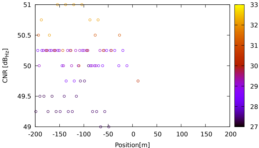
CNR vs position for G04 (L5) on LeicaGS18 - DOY 262 jam. 2
