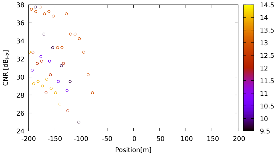
CNR vs position for G08 (L1) on LeicaGS18 - DOY 262 jam. 2
