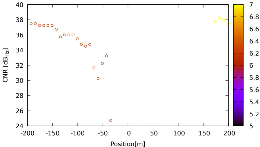
CNR vs position for G08 (L1) on LeicaGS18 - DOY 262 jam. 3
