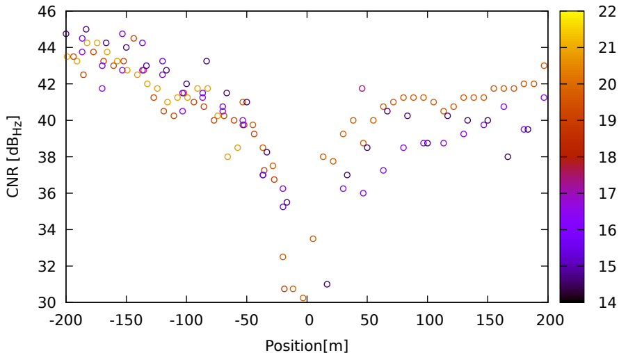
CNR vs position for G08 (L5) on LeicaGS18 - DOY 262 jam. 1
