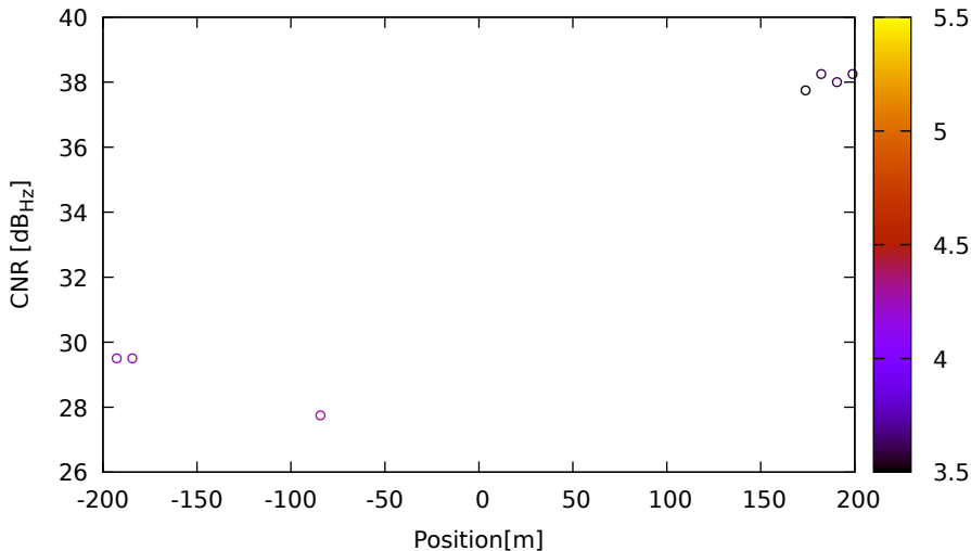
CNR vs position for G09 (L1) on LeicaGS18 - DOY 262 jam. 3
