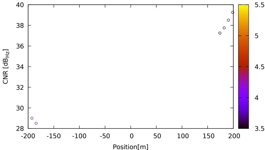
CNR vs position for G09 (L2) on LeicaGS18 - DOY 262 jam. 3
