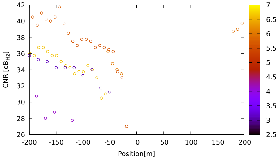
CNR vs position for G14 (L5) on LeicaGS18 - DOY 262 jam. 1
