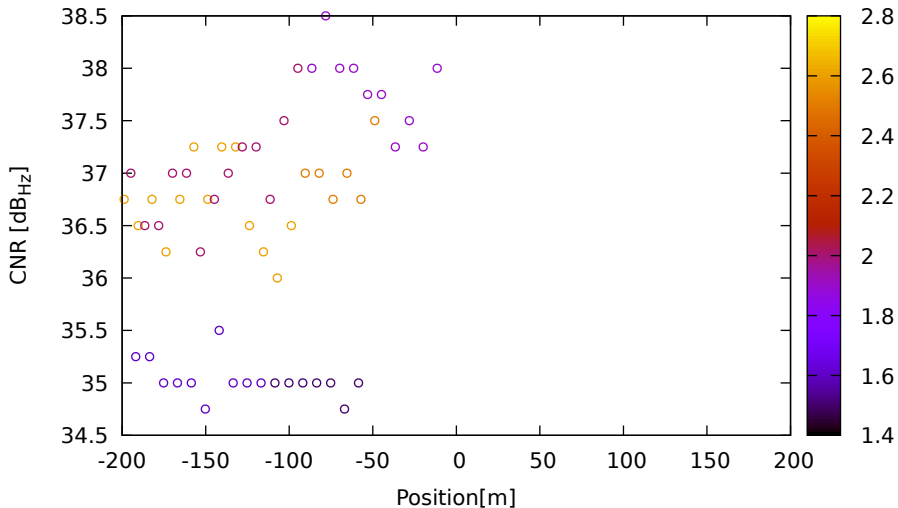
CNR vs position for G14 (L5) on LeicaGS18 - DOY 262 jam. 2
