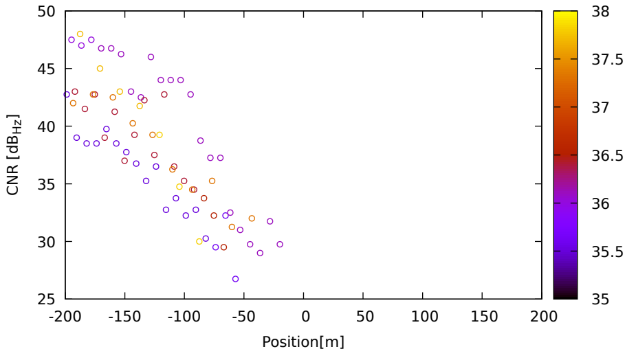
CNR vs position for G17 (L1) on LeicaGS18 - DOY 262 jam. 2
