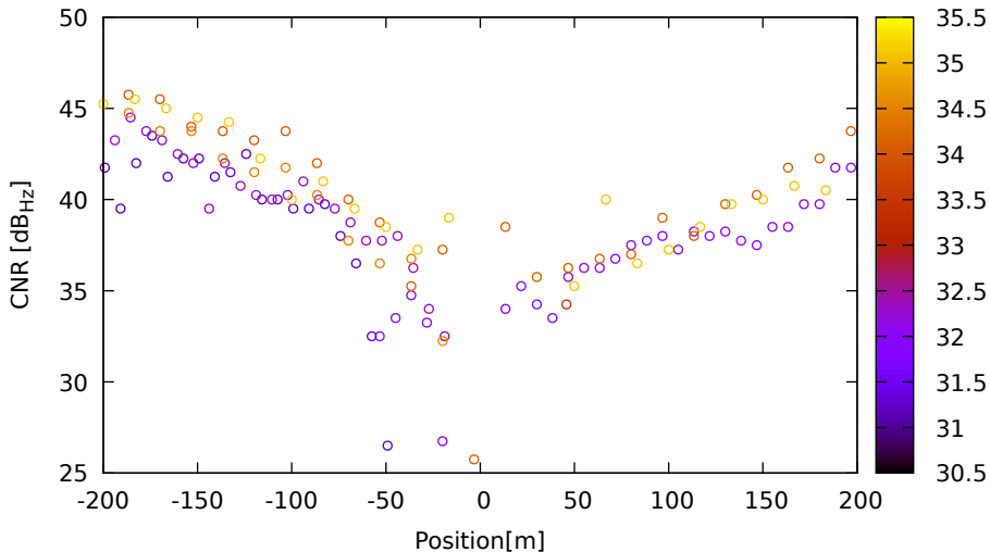
CNR vs position for G17 (L2) on LeicaGS18 - DOY 262 jam. 1
