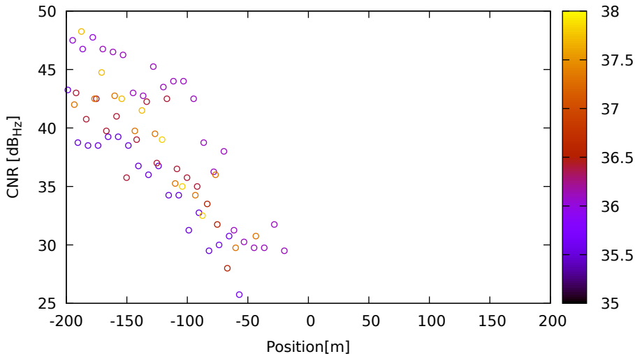
CNR vs position for G17 (L2) on LeicaGS18 - DOY 262 jam. 2
