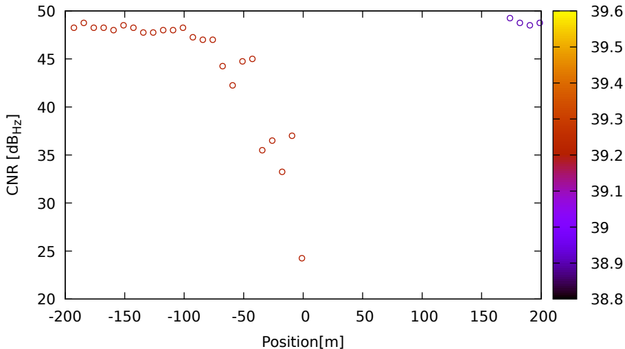
CNR vs position for G17 (L2) on LeicaGS18 - DOY 262 jam. 3
