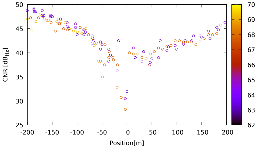
CNR vs position for G21 (L1) on LeicaGS18 - DOY 262 jam. 1
