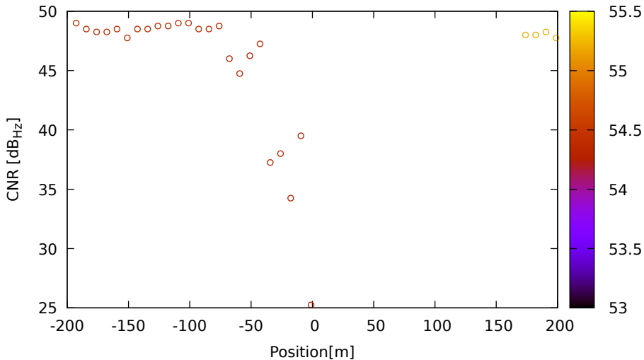
CNR vs position for G21 (L2) on LeicaGS18 - DOY 262 jam. 3
