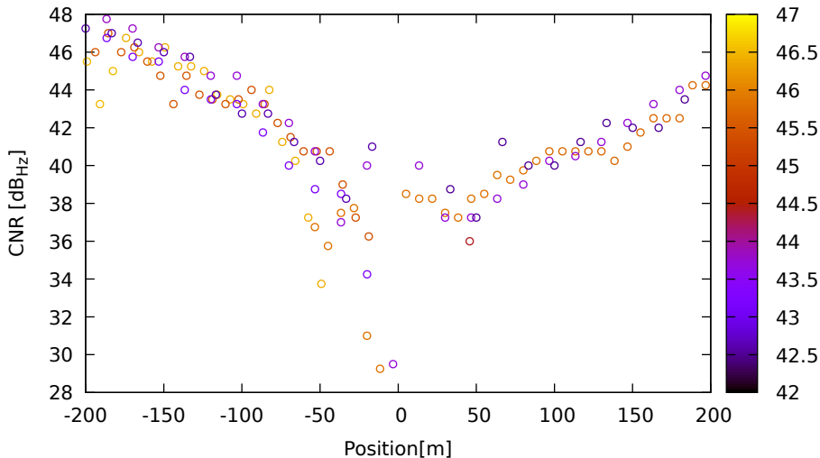
CNR vs position for G22 (L1) on LeicaGS18 - DOY 262 jam. 1
