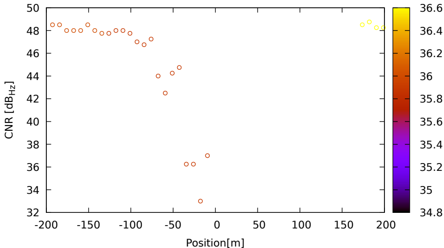
CNR vs position for G22 (L1) on LeicaGS18 - DOY 262 jam. 3
