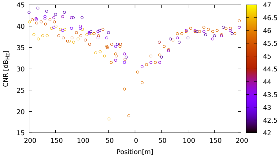
CNR vs position for G22 (L2) on LeicaGS18 - DOY 262 jam. 1
