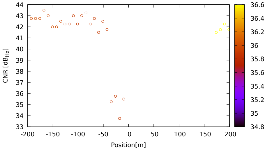
CNR vs position for G22 (L2) on LeicaGS18 - DOY 262 jam. 3
