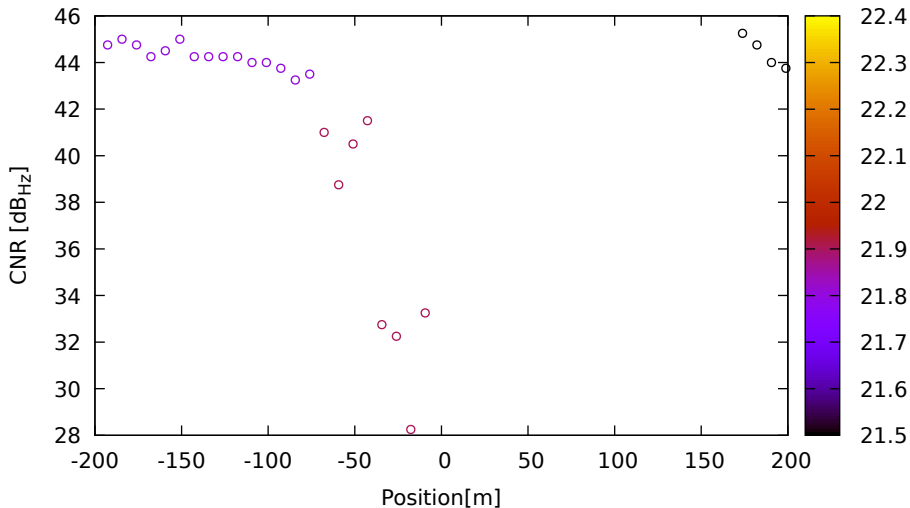
CNR vs position for G31 (L1) on LeicaGS18 - DOY 262 jam. 3
