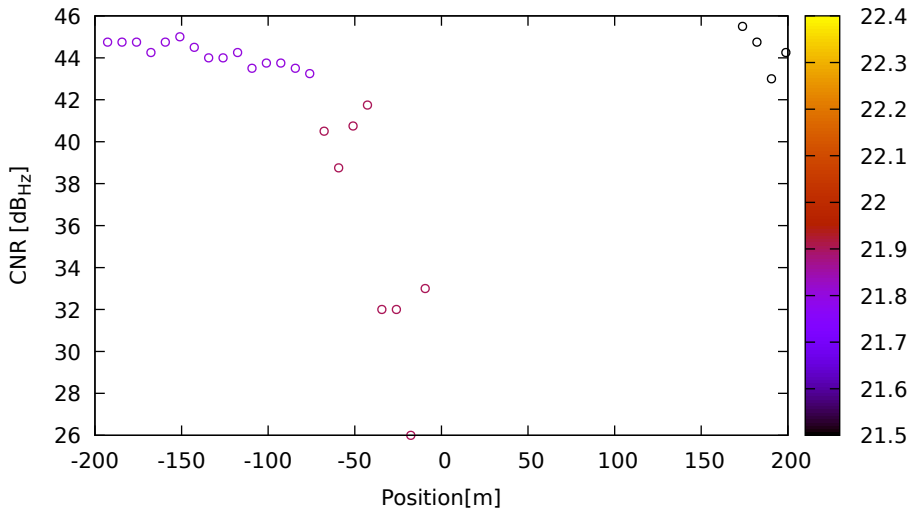
CNR vs position for G31 (L2) on LeicaGS18 - DOY 262 jam. 3
