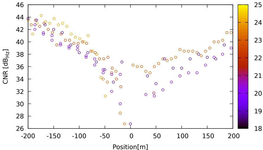
CNR vs position for G32 (L1) on LeicaGS18 - DOY 262 jam. 1
